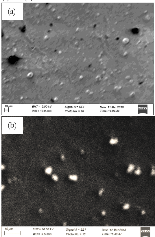
Figure 5: SEM image of (a) 15 wt % TiO 2 films annealed at 450 °C and (b) 20 wt % TiO 2 films annealed at 500 °C.
