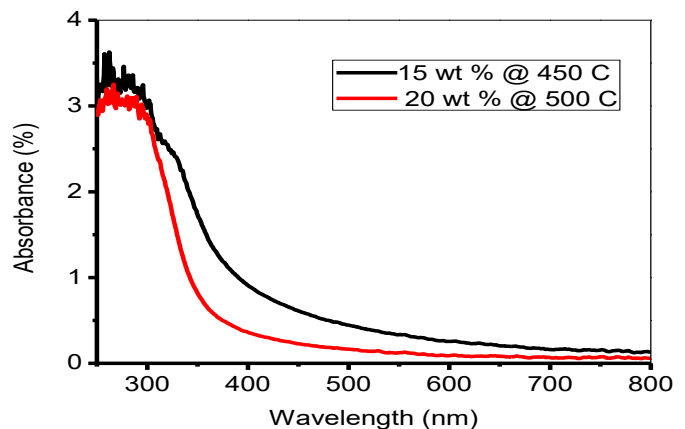
Figure 3: Plot of absorbance versus wavelength of 20 wt % and 15 wt % samples of \text{TiO}_2 films annealed at 450^\circ\text{C} and 500^\circ\text{C} .
